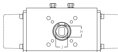
Top view model 032 – 240
